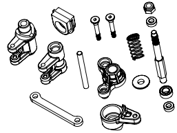
500406040 Servosaver/Lenkhebel-Set Servo saver / steering arm set
